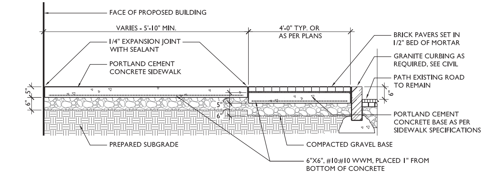
I TYPICAL STREETSCAPE SECTION L7.0 1/2" = 1'-0" SECTION
